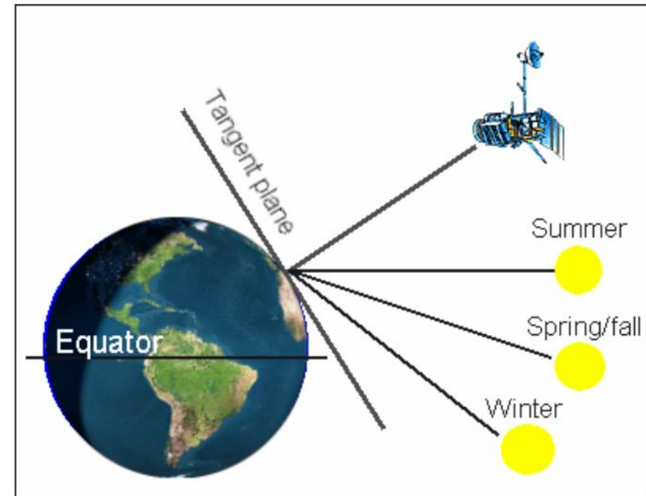
Sun elevation difference per season (adapted from Lillesand and Kiefer, 2015)
